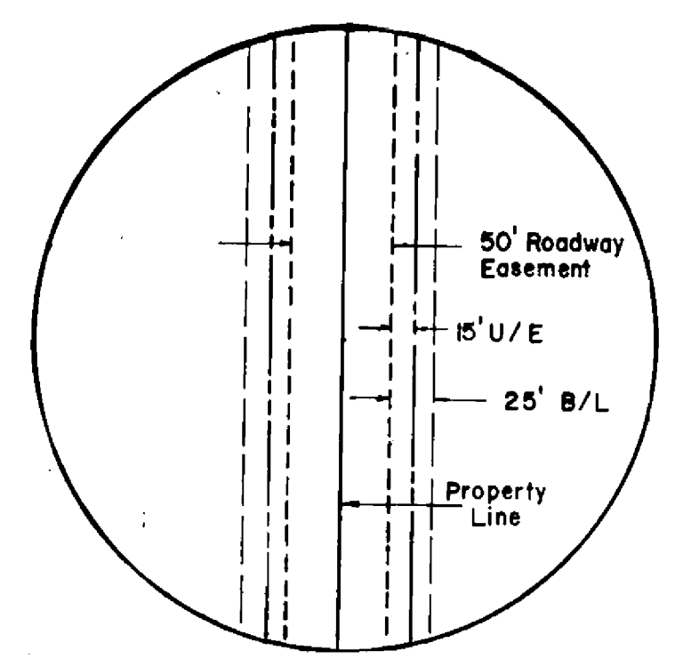
TYPICAL EASEMENT LAYOUT
