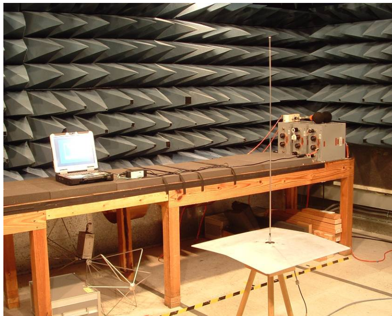
Rod Antenna, 2 to 30 MHz
