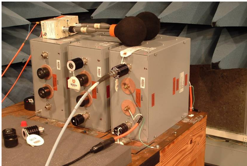
Measurement on High Side of Power
