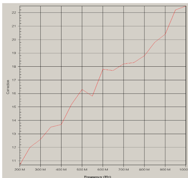
EMCO 3106 Double Ridge Guide
