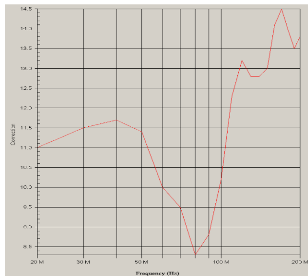
EMCO 3109 Biconical
