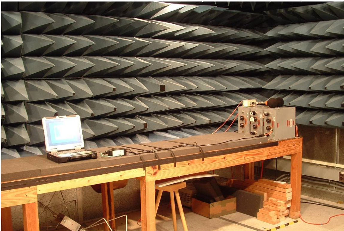
General Test Setup
