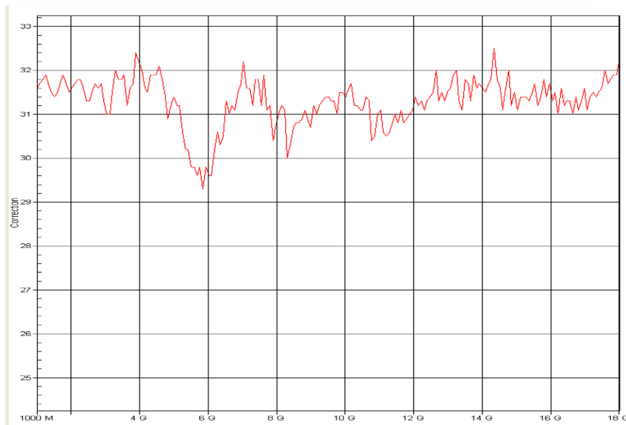
Mitek 1429606 Gain, 1 to 18 GHz
