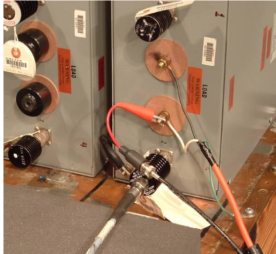
Signal Injection for Calibration on Low side of Power
