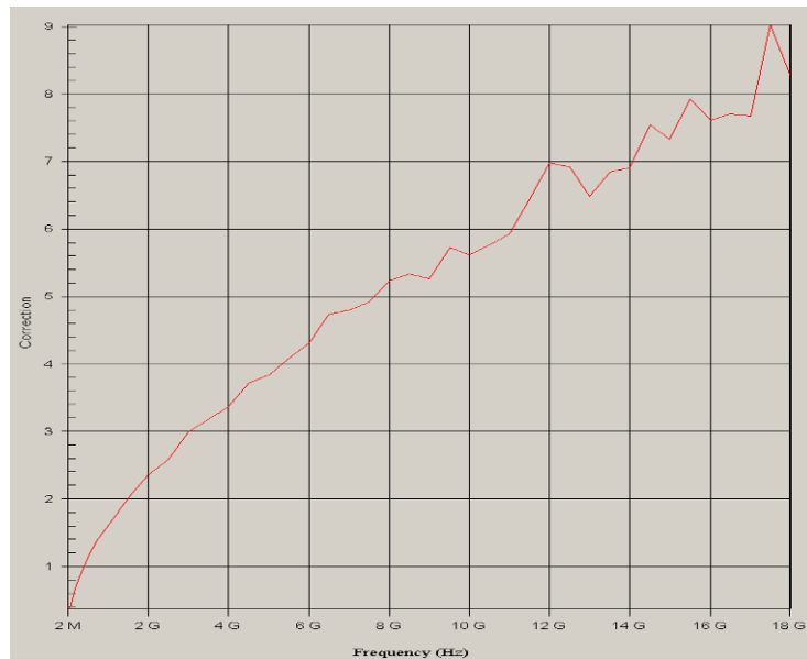
Cable Loss - Semflex Coax
